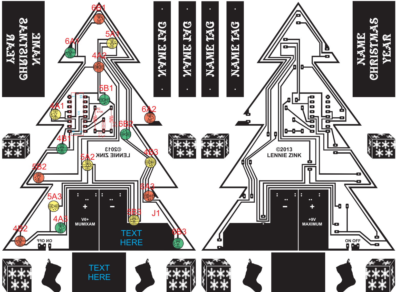
COMPONENT LAYOUT
